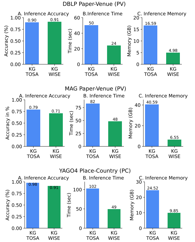
Fig. 9. KG-TOSA vs. KG-WISE on node classification tasks using three metrics: (A) Inference Accuracy (higher is better), (B) Inference Time (lower is better), and (C) Inference Memory (lower is better). Our LLM-guided subgraph extraction and query-aware inference substantially improve efficiency: KG-WISE reduces inference time by 41–52% and memory usage by 60–84% while preserving accuracy.
