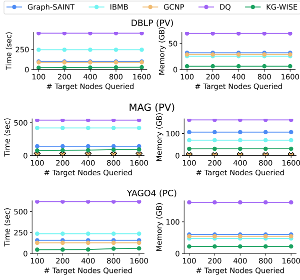
Fig. 12. Node classification inference time and memory usage of KG-WISE compared to SOTA GNN accelerators as the number of target nodes per query increases. The top, middle, and bottom rows correspond to the DBLP, MAG, and YAGO NC tasks, respectively. KG-WISE exhibits superior performance in all cases.
