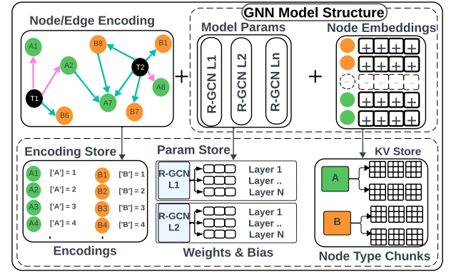
Fig. 3. The top half shows an encoded KG and a GNN trained on it. The GNN’s main components are the learned parameters and non-target node embeddings . The bottom half illustrates how KG-WISE maps the encoding and decouples the GNN components. The node embeddings are stored in a key-value store as row-wise chunks grouped by node type in a Zarr KV store.
