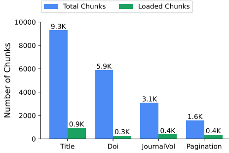
Fig. 10. The number of KV-store chunks loaded per node type by KG-WISE to answer the 1K target node inference query on the DBLP KG. KG-WISE loaded just 10% of the KV chunks, achieving significant savings in both
