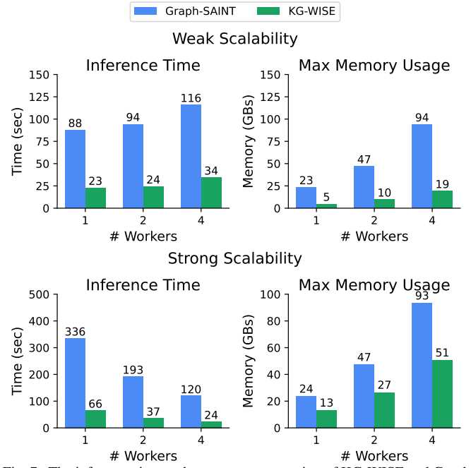
Fig. 7. The inference time and memory consumption of KG-WISE and Graph-SAINT inference pipelines under weak and strong scalability settings. KG-WISE shows better scalability in both settings.
