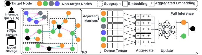
Fig. 1. A GNN inference query for target nodes (TN) loads the KG’s adjacency, model, and embedding matrices from storage, then performs message passing and embedding updates to produce predictions. This process is resource-intensive and scales poorly with the size of these matrices in KGs.
